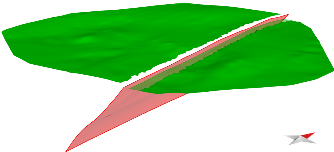
Figure 6. Preview of the Upper Cretaceous footwall area to be snapped to Fault 2.
