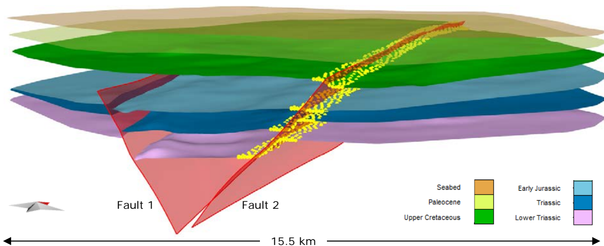
Figure 1: Model derived from a North Sea dataset. Surfaces filtered using the Query tool for locations where the distance to Fault 2 is <300 m. Yellow points correspond to the selected vertices.
