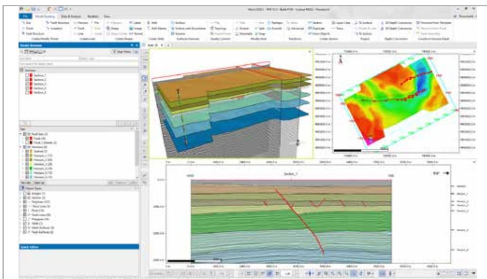
3D model at Penobscot of the Sable sub-basin, offshore Nova Scotia © Department of Natural Resources Canada. All rights reserved.
