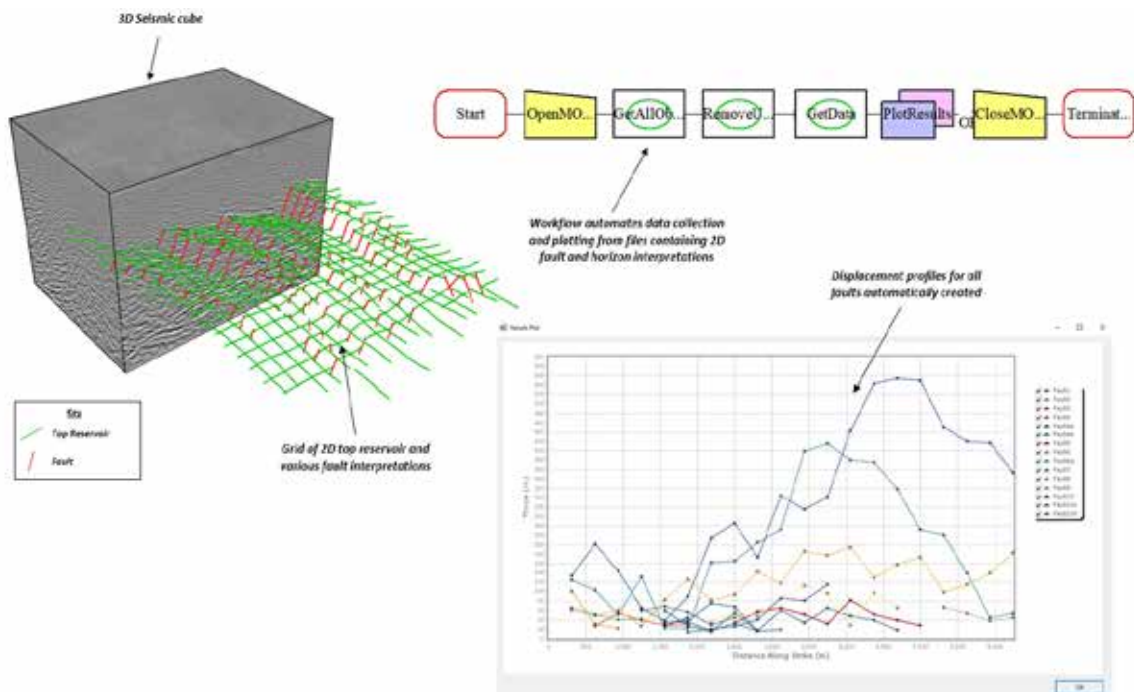
Automated creation of fault displacement profiles from 2D section interpretations.
